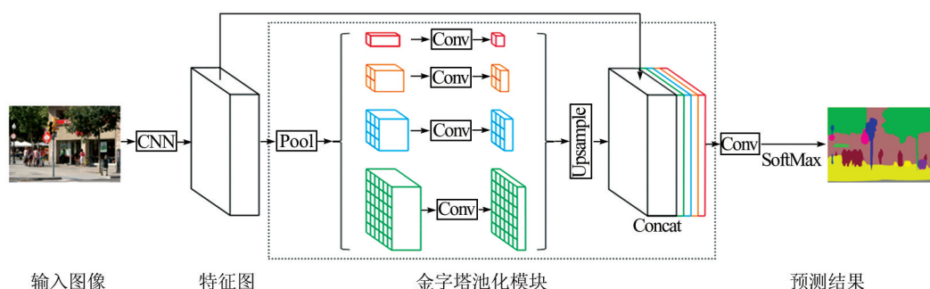
图12 PSPNet框架 [29]
